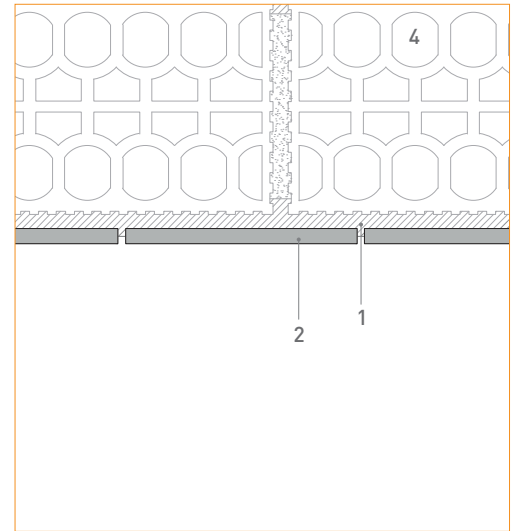
2. Horizontal detail
