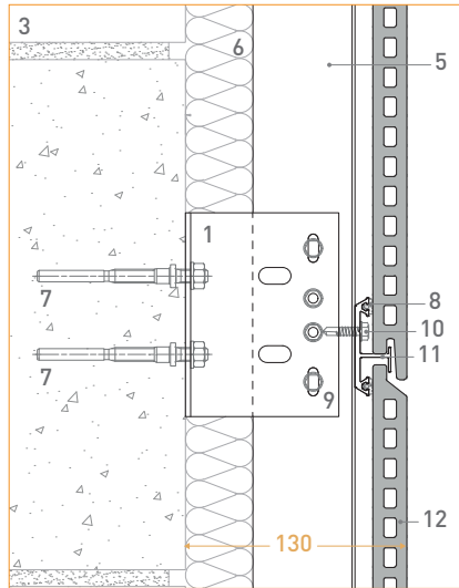
1. Support bracket
