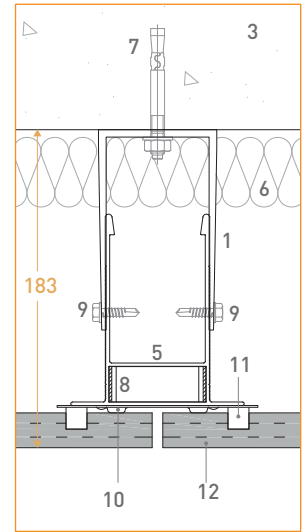
3. Horizontal detail
