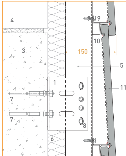
1. Support bracket
