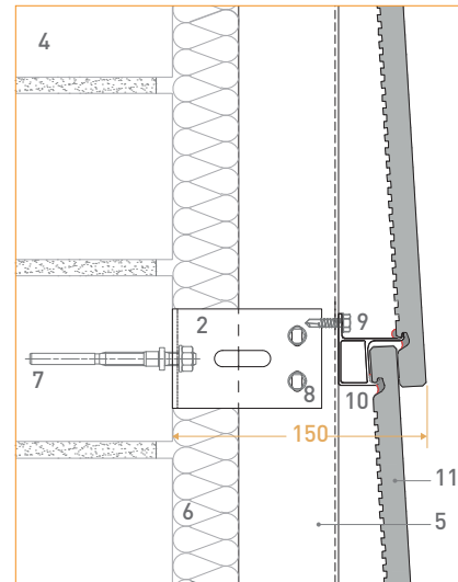
2. Stop bracket
